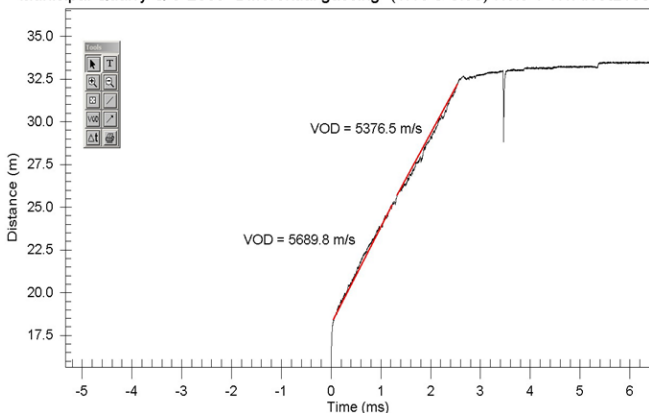
Municipal Quarry Q-9-2009 Differential gassing (1.10 & 0.95) Hole 1 TITAN XL1000
